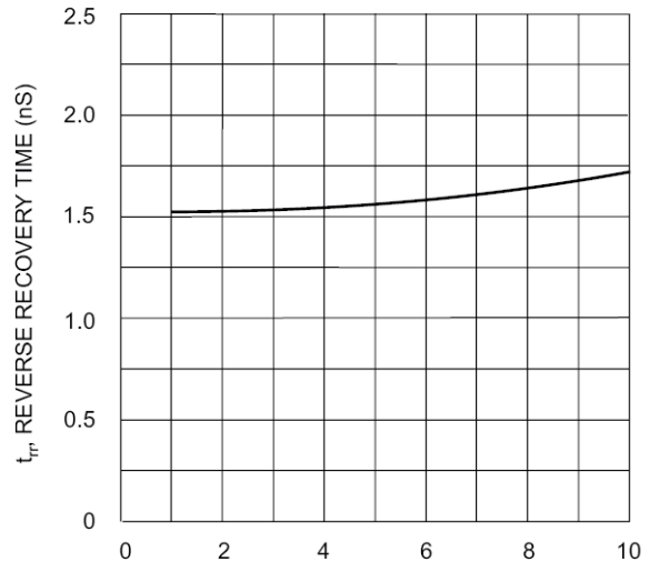
Fig. 4 Reverse Recovery Time vs. Forward Current
